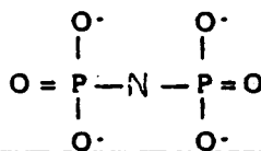
Nitrobisphosphonate
